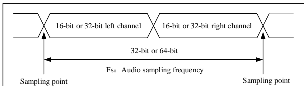
Figure 21-26 Audio sampling frequency definition
