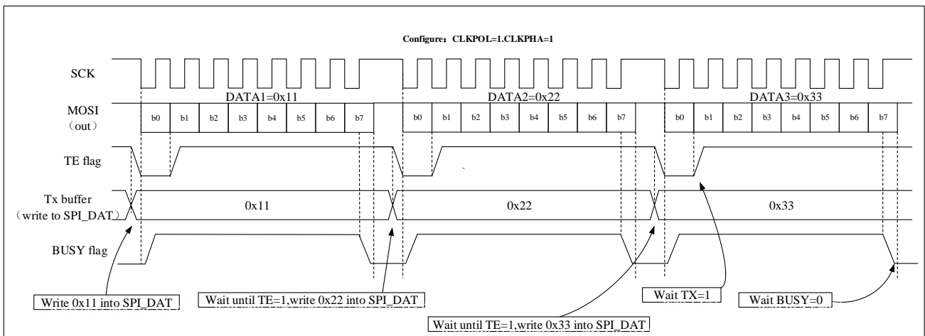
Figure 21-10 Schematic diagram of TE/BUSY change when BIDIRMODE = 0 and ROONLY = 0 are transmitted discontinuously.
